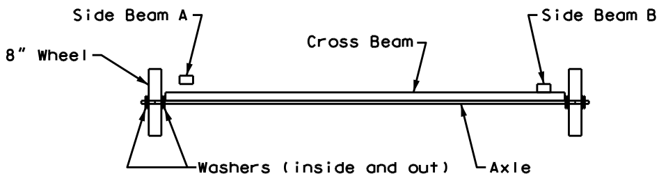
SECTION ALONG AXLE
